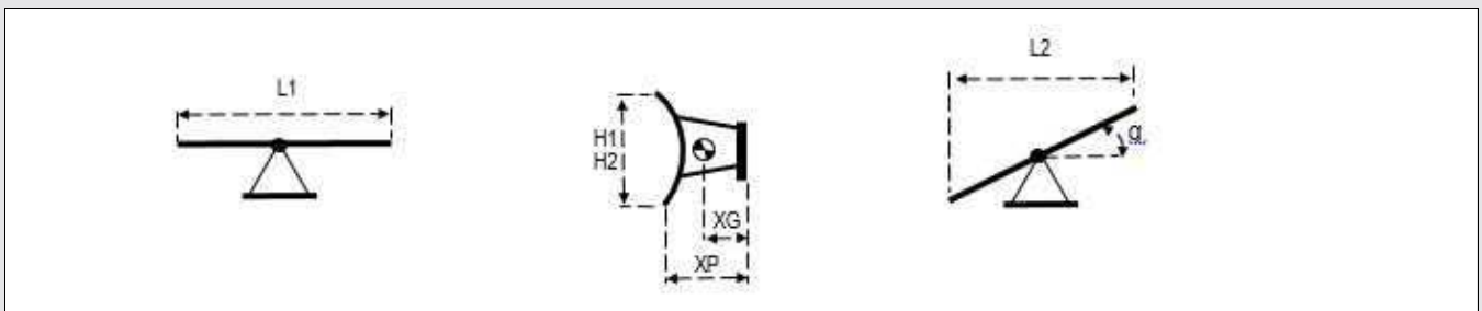
Oscillation
